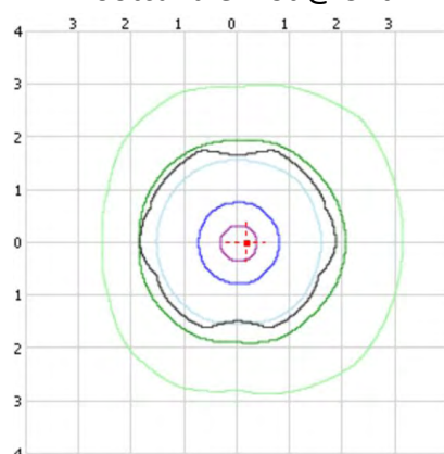
Footcandle Plot @ 9 ft
